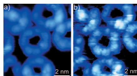
Figure 3. Bias dependent STM images of \text{Mo}_{154} clusters deposited on Au(111). a) Positive sample voltage ( V_{\text{sample}}=3 V, I=5 pA) showing the spatial distribution of the unoccupied states. b) Negative sample voltage ( V_{\text{sample}}=-2 V, I=5 pA) showing the spatial distribution of the occupied states.
