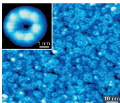
Figure 2. Constant current STM image of wheel shaped \text{Mo}_{154} clusters deposited on Au(111) ( V_{\text{sample}}=3 V, I=5 pA). Inset: high-resolution STM image of the \text{Mo}_{154} cluster exhibiting sevenfold rotational symmetry with seven bright protrusions on the ring ( V_{\text{sample}}=3 V, I=2 pA).
